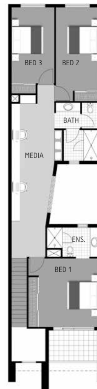
GROUND FLOOR
